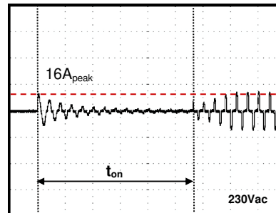
(Fig.8 inrush with an ESB)
